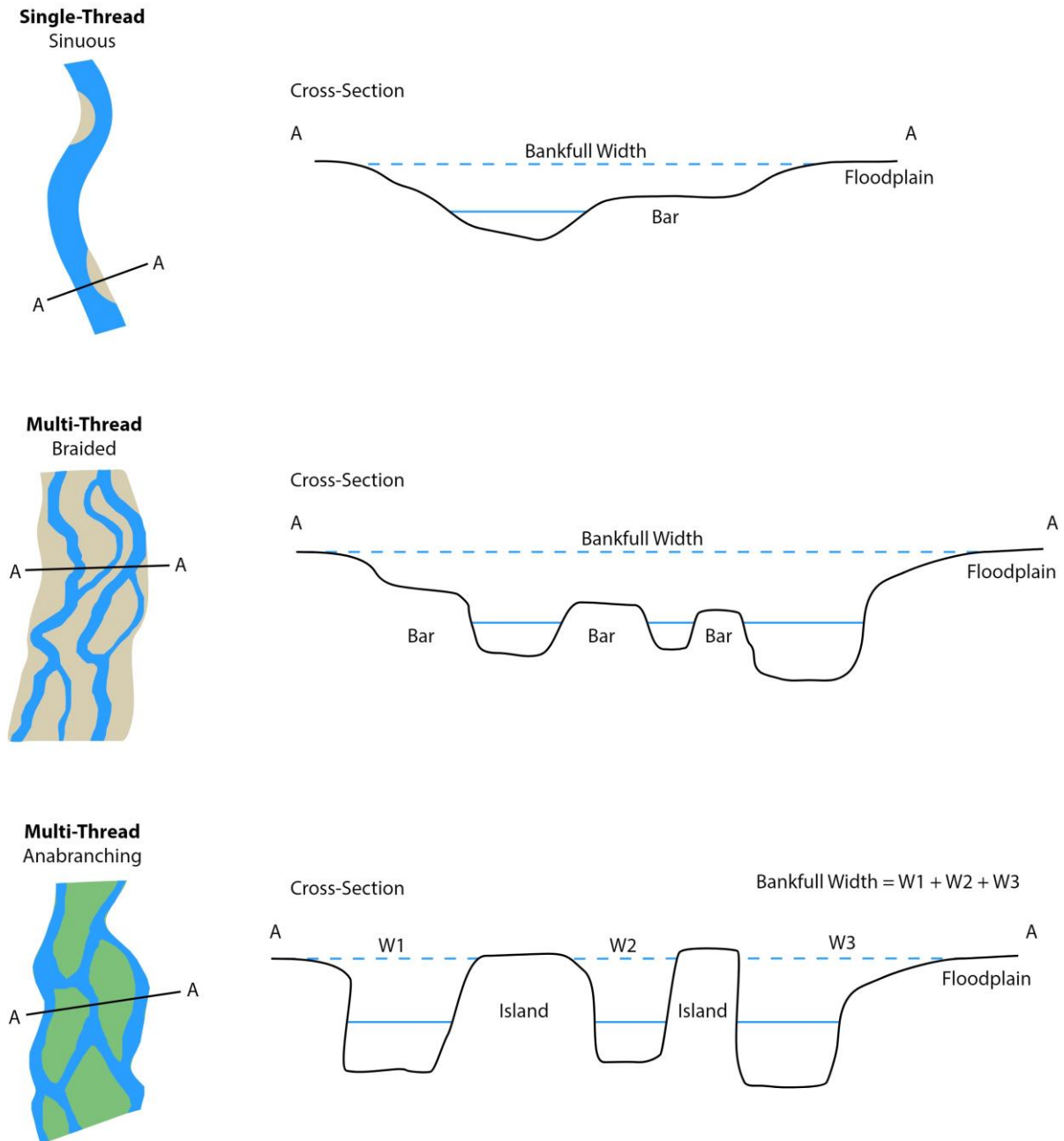
Figure 3 - Identification of the bankfull width in different river types. The water surface refers to normal water channel conditions (plan view on the left and continuous light blue line on the right) or bankfull conditions (dashed light blue line on the right).
