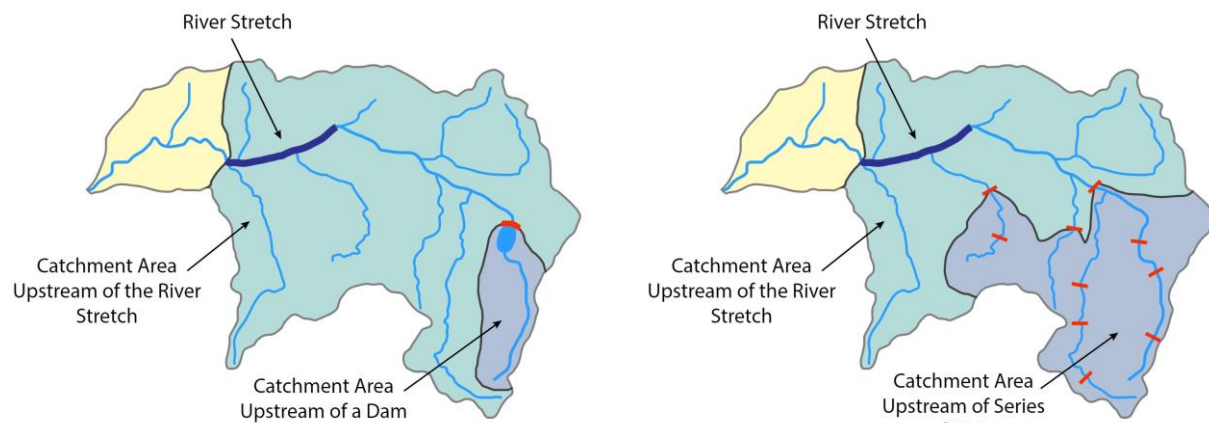
Figure 5 - Example of how to consider and compute the severity of barriers' sediment load interception in the case of (left) a dam and (right) a series of weirs
